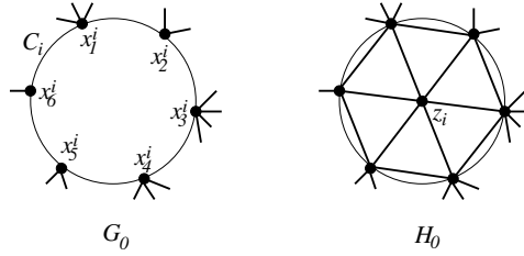
Fig. 1. From G_0 to H_0
